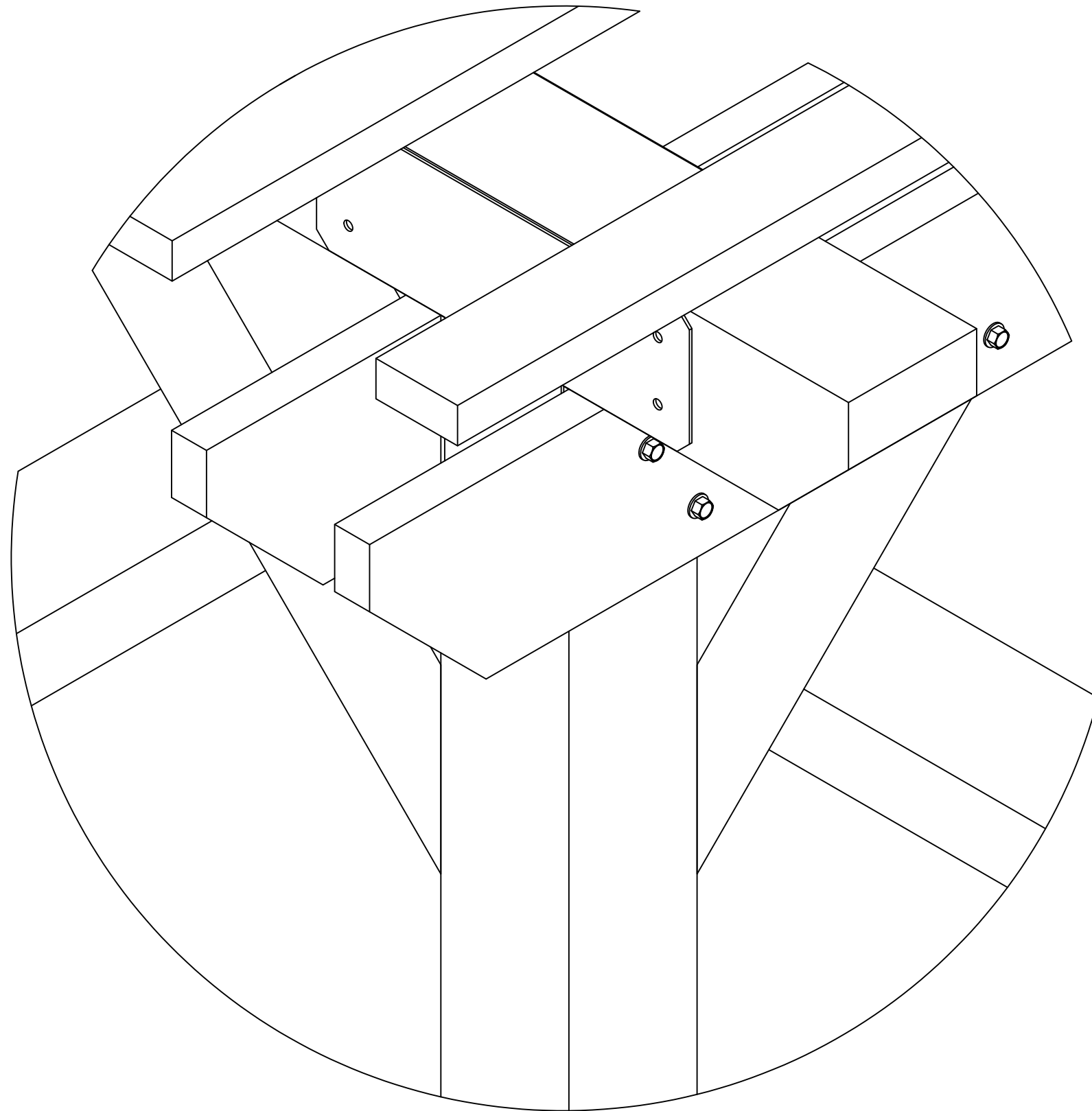
DETAIL C SCALE 3" = 1'-0"
